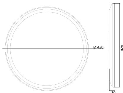
24W Ø420x30mm
