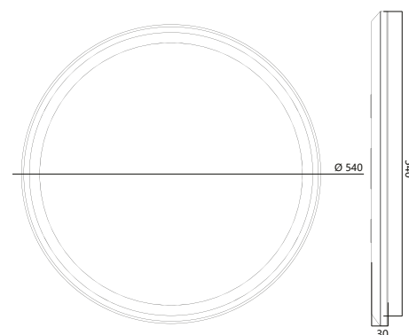
32W Ø540x30mm
