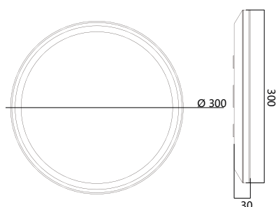
18W Ø300x30mm
