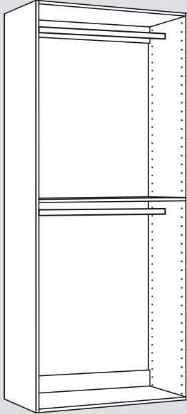
2048H x 750W x 380D 1x Cabinet Shell I/N: 0430466 2x Hanging Rail I/N: 0431022 bundle0631
