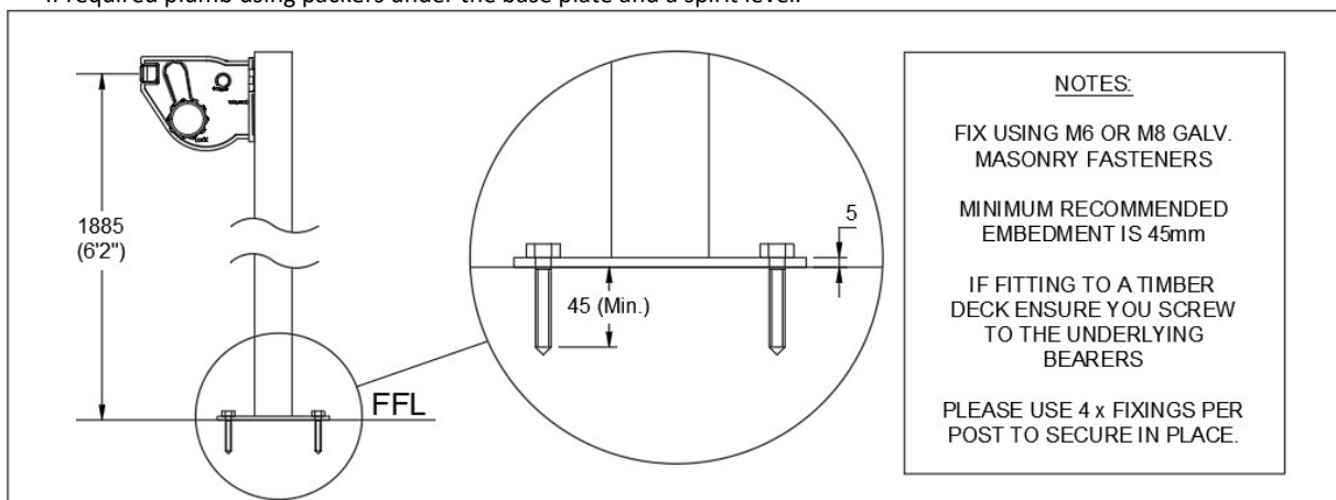
Fig. 9 Installation of Plated Post.
