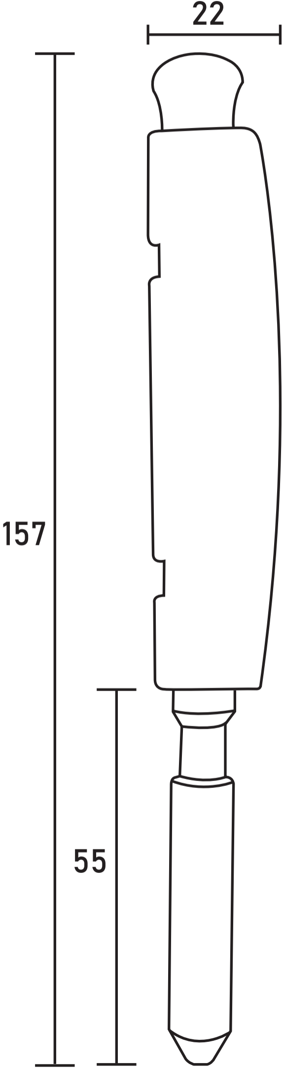
SIDE VIEW
