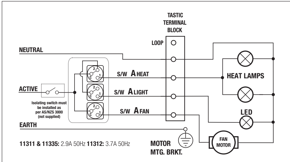
Fig. 7: Wiring diagram for model 11311, 11312 and 11335.
