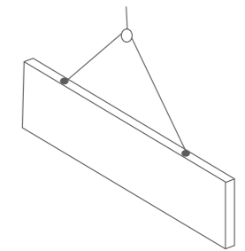
45MPa Concrete Strength Rigging Angle 60°
