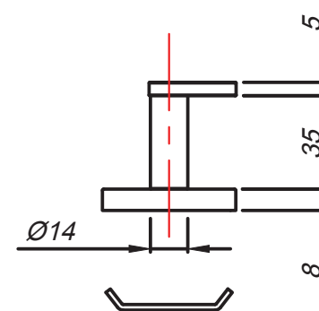
Mounting Plate
