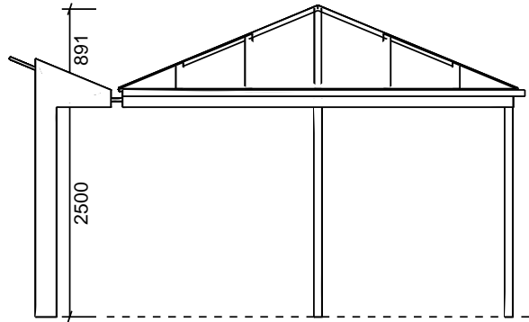
FRONT ELEVATION 1:75
