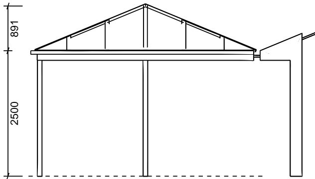
BACK ELEVATION 1:75
