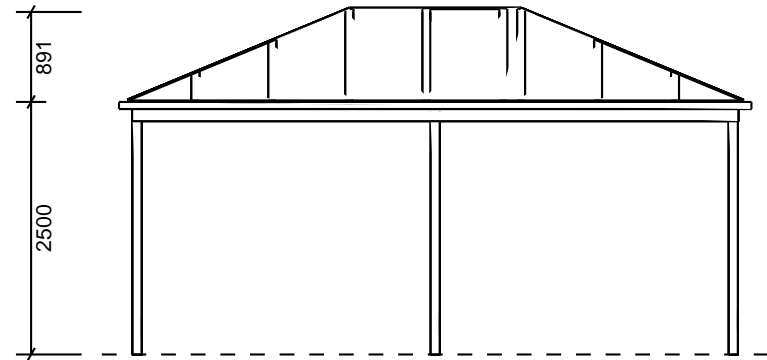
RIGHT ELEVATION 1:75
