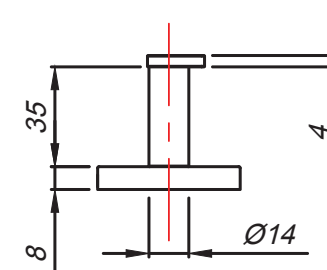
Mounting Plate
