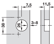
Hinge Drilling Pattern
