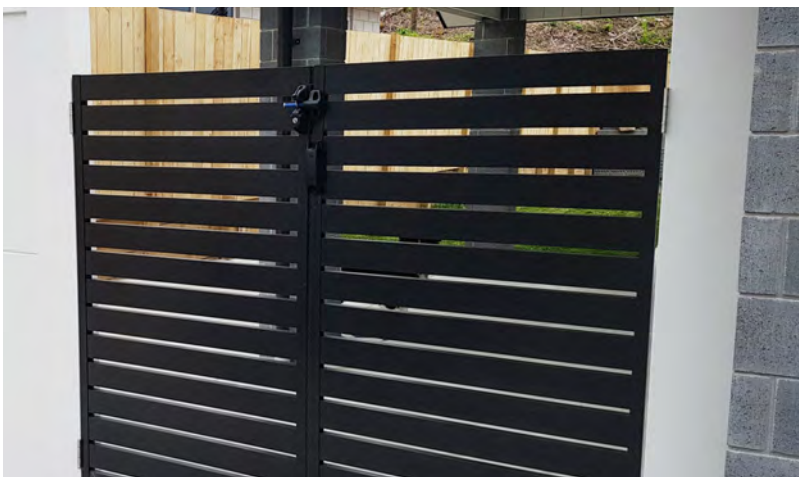
GATE POST - 90mm x 90mm in-ground or flanged + flush fit post cap
