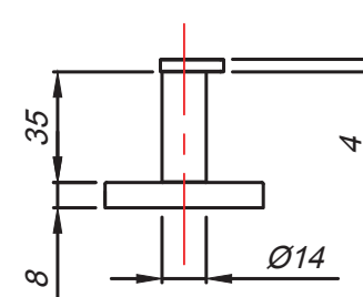
Mounting Plate
