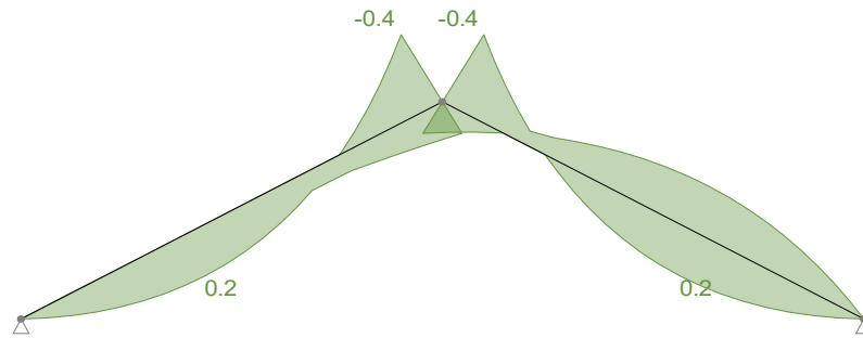
Strength combinations - Moment envelope (kNm)
