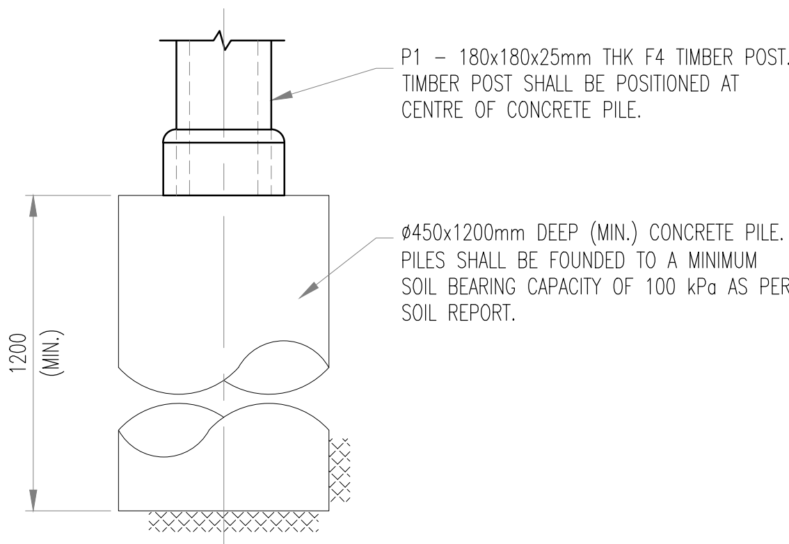
TYPICAL PILE DETAIL SCALE: 1:10
