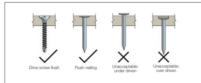
FASTENER DEPTH
