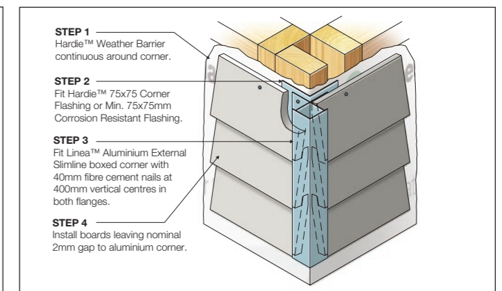
FIGURE 6 EXTERNAL CORNER SLIMLINE BOX CORNER OPTION
