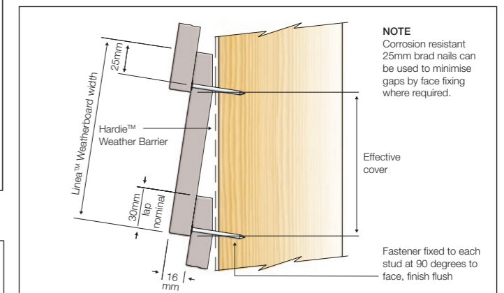
FIGURE 3 CONCEALED FIXING OPTION
