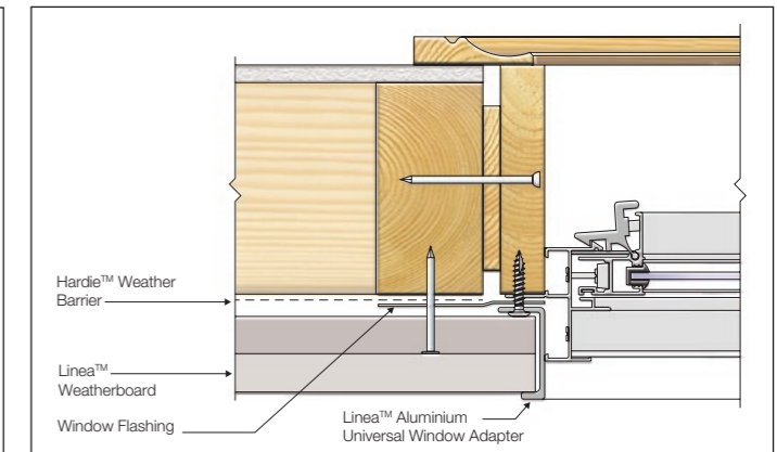
FIGURE 17 WINDOW JAMB - LINEA™ WINDOW ADAPTER OPTION
