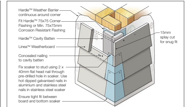
FIGURE 8 EXTERNAL CORNER SOAKERS OPTION
