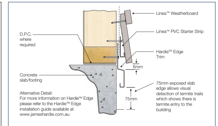
FIGURE 2 SLAB JUNCTION ALTERNATIVE
