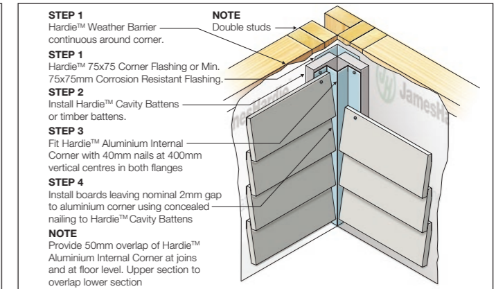
FIGURE 11 INTERNAL CORNER MOULD OPTION
