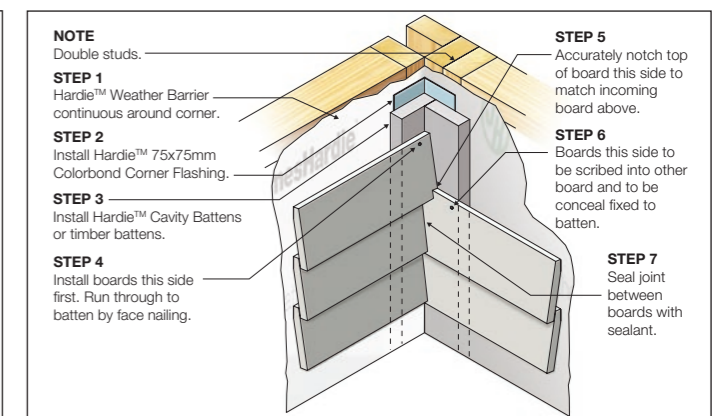
FIGURE 13 INTERNAL CORNER NOTCH & SCRIBE OPTION
